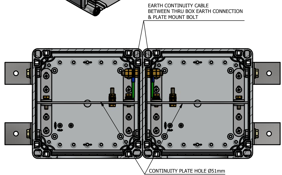
SECTION A-A LID REMOVED
